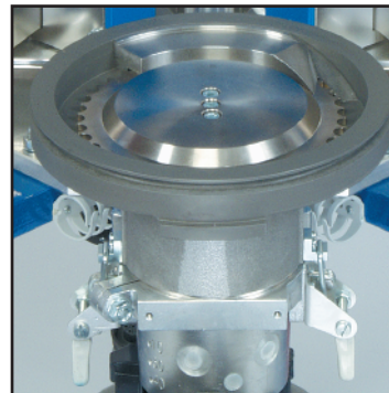
A properly sized dosing disc provides high performance at feed rates below 50 g/hr (0.1 lbs./hr)
