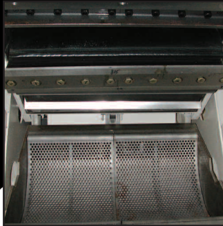
Tangential feed cutting chamber allowing for better ingestion of feedstock
